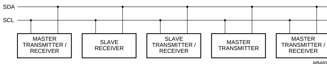
Fig.6 System configuration.
