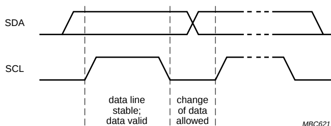
Fig.4 Bit transfer.
